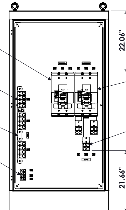
FRONT VIEW DOOR/DEADFRONT REMOVED
