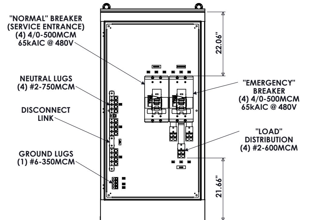
FRONT VIEW DOOR/DEADFRONT REMOVED
