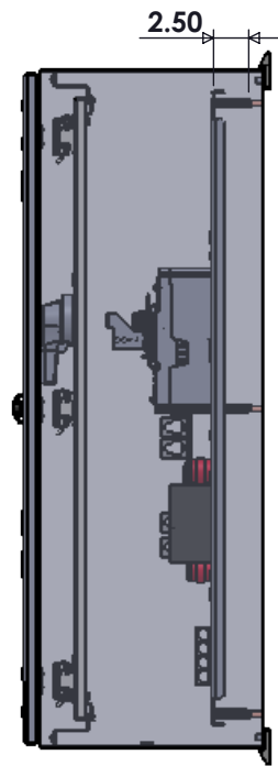
SIDE VIEW
