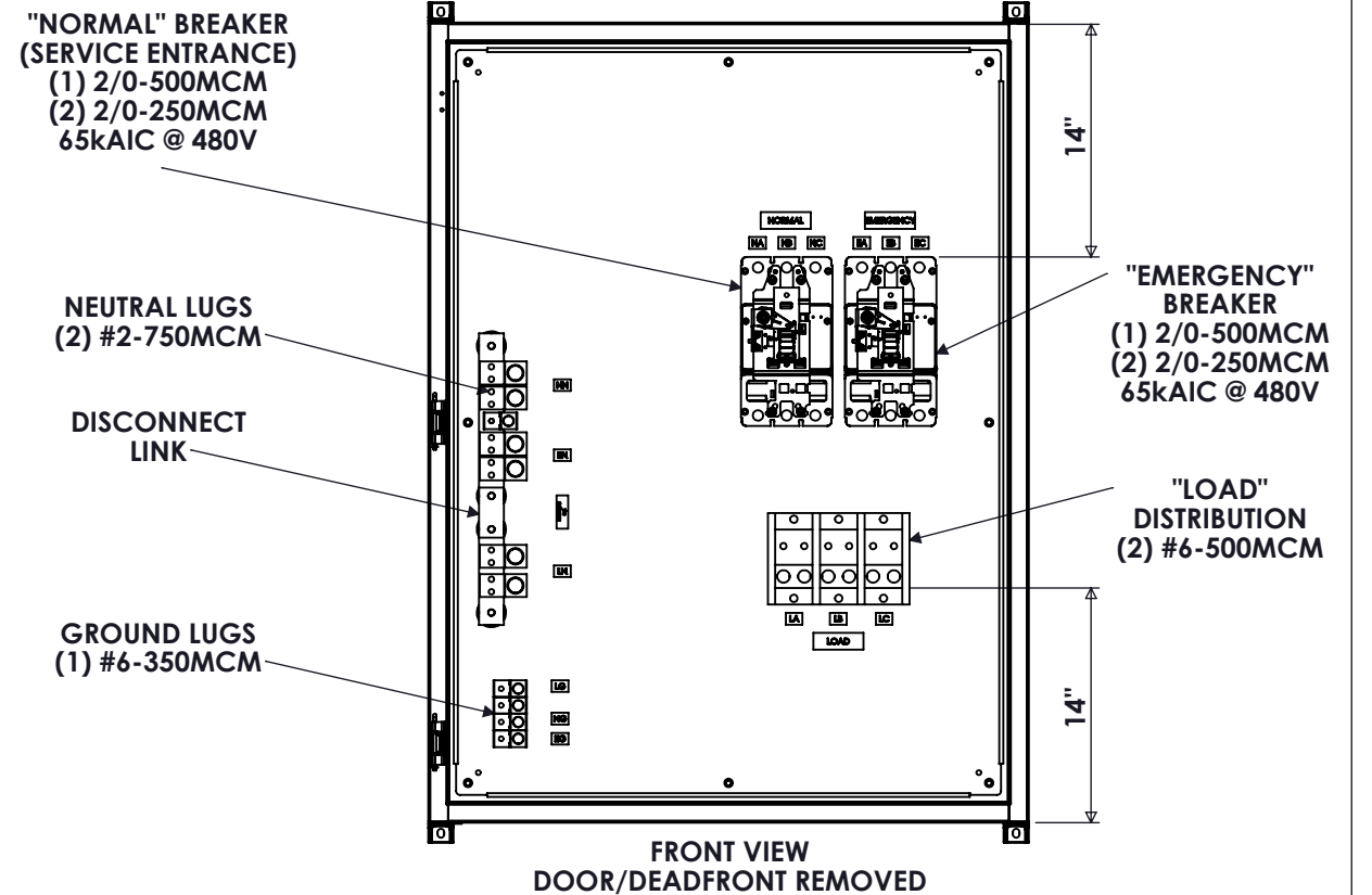
FRONT VIEW DOOR REMOVED
