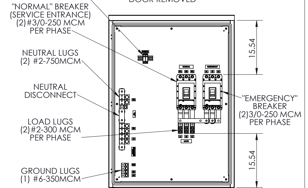
FRONT VIEW DOOR/DEADFRONT REMOVED
