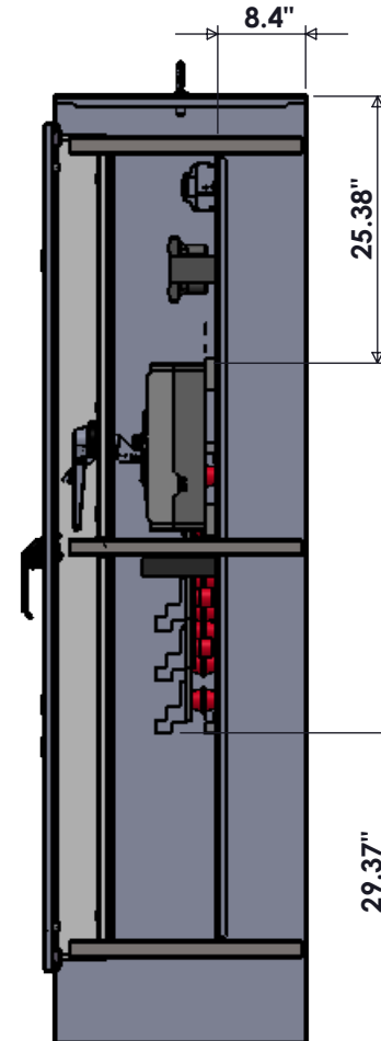
SIDE VIEW
